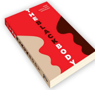
THE BLACK BODY
